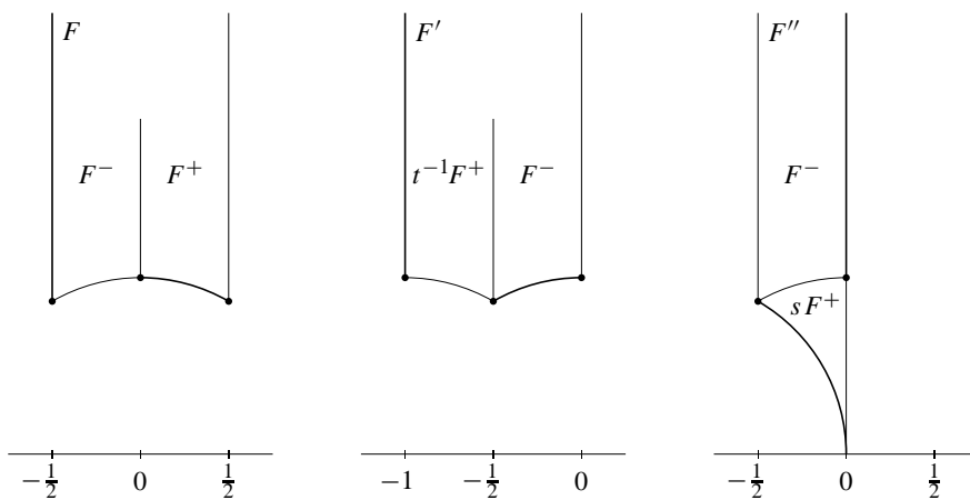
The fundamental domains F, F' and F'' for \Gamma(1) .
