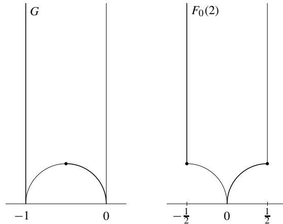
The fundamental domains G and F_0(2) for \Gamma_0(2) .
