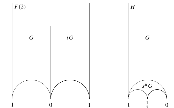
The fundamental domains F(2) and H for \Gamma(2) .
