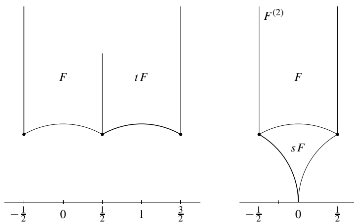
Fundamental domains for \Gamma^{(2)} .
