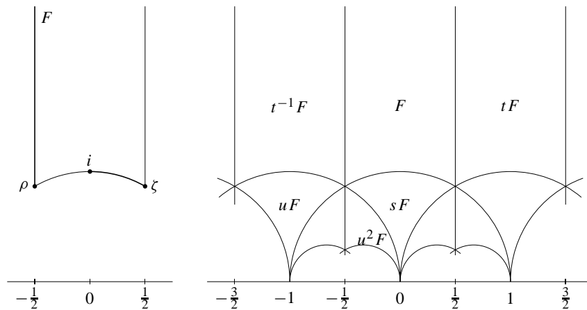
The fundamental domain F for \Gamma(1) , and some of its transforms.
