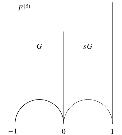
The fundamental domain F^{(6)} for \Gamma^{(6)} .
