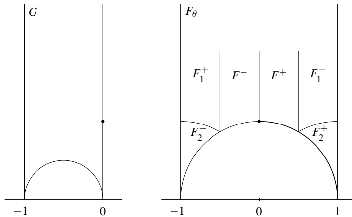
The fundamental domains G and F_\theta for \Gamma_\theta .
