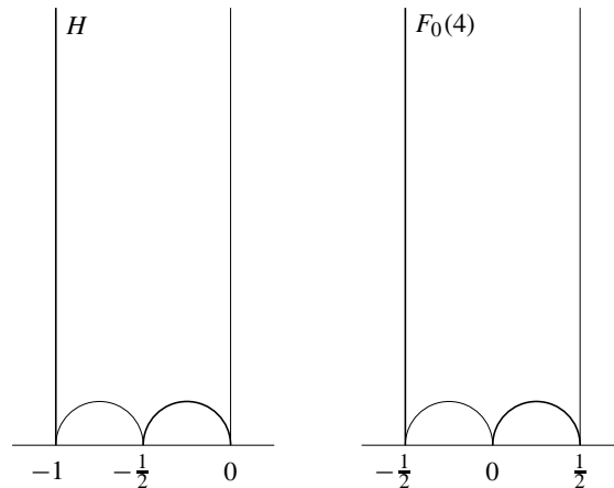
The fundamental domains H and F_0(4) for \Gamma_0(4) .
