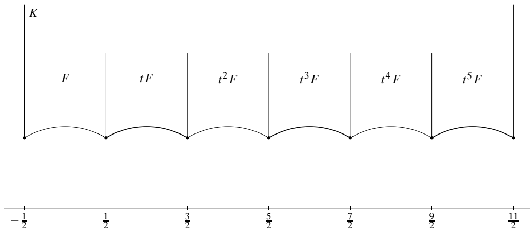
The fundamental domain K for \Gamma^{(6)} .
