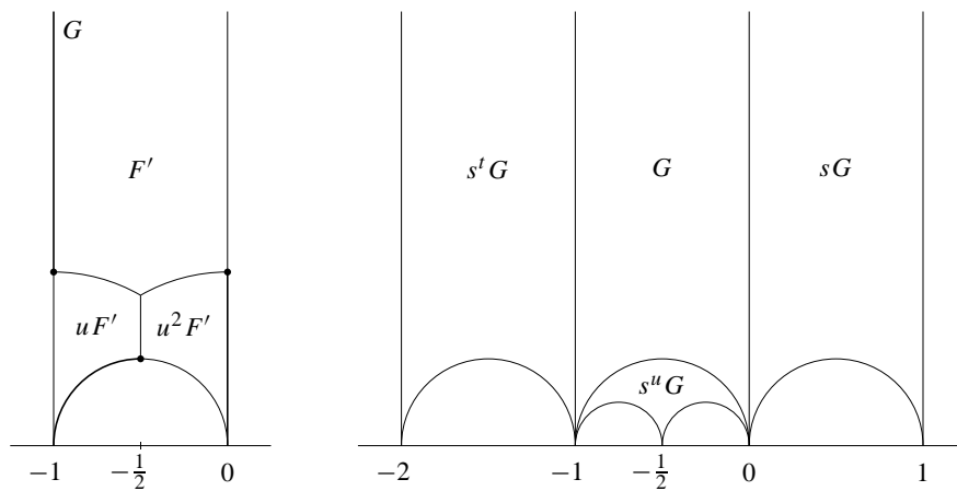
The fundamental domain G for \Gamma^{(3)} , and some of its transforms.
